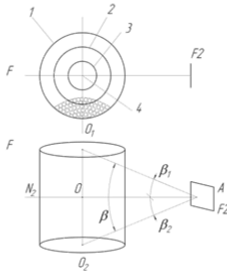
Figure4. Radiation of cylindrical gas volume on the calculated area F_2
